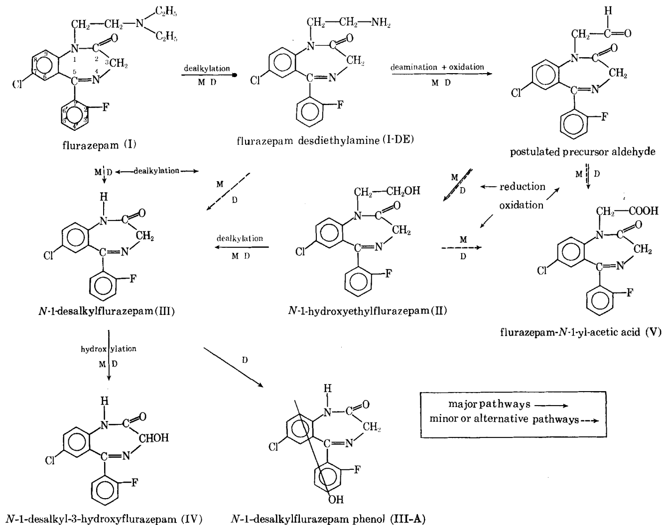
N-1-desalkyl-3-hydroxyflurazepam (IV) N-1-desalkylflurazepam phenol (III-A) Scheme III—Postulated metabolic pathways of flurazepam in man (M) and in dog (D)
